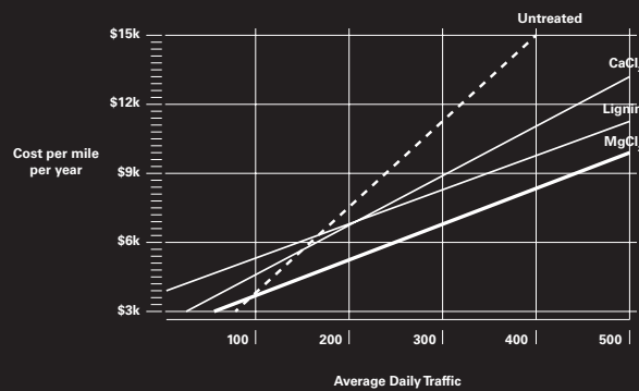
COST OF TREATMENT vs. AVERAGE DAILY TRAFFIC (ADT) @ AGGREGATE COST OF $11.57 / TON IN PLACE
